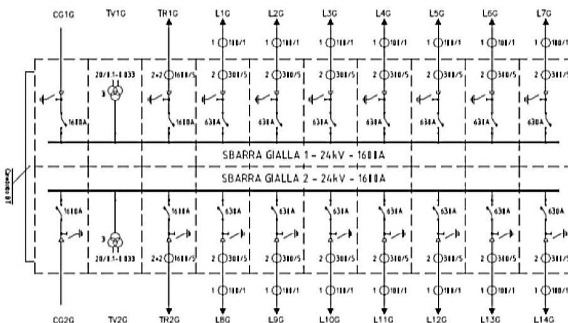
Figura 41. CONTAINER DY770E/3.Unifilar
